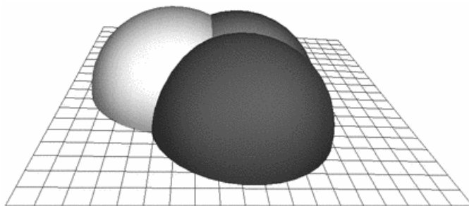
FIGURE 1. Three hemispheres intersecting at a point.
